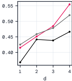
RMSE (%)
